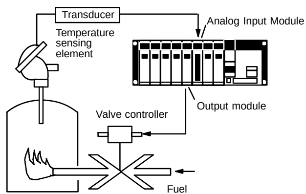
Furnace Control with Analog Input
